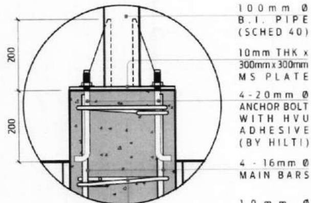
SPOT DETAIL - B
