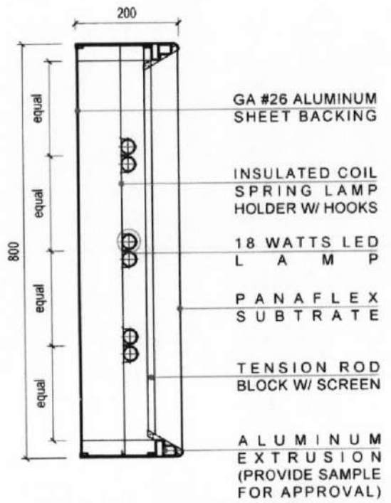
BLOW-UP SECTION-2 SCALE: 1:10 M
