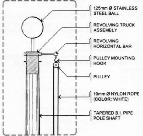
1b SPOT DETAIL - A SCALE 1:10 METERS
