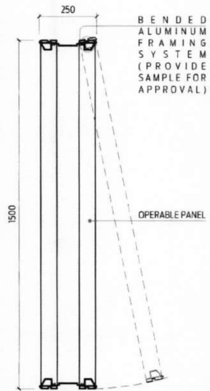
SECTION - B
