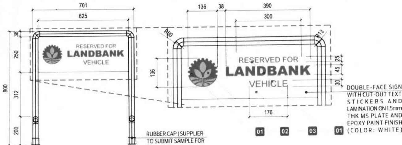
BLOW-UP DETAIL
