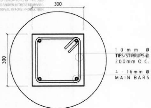
SPOT DETAIL - A
