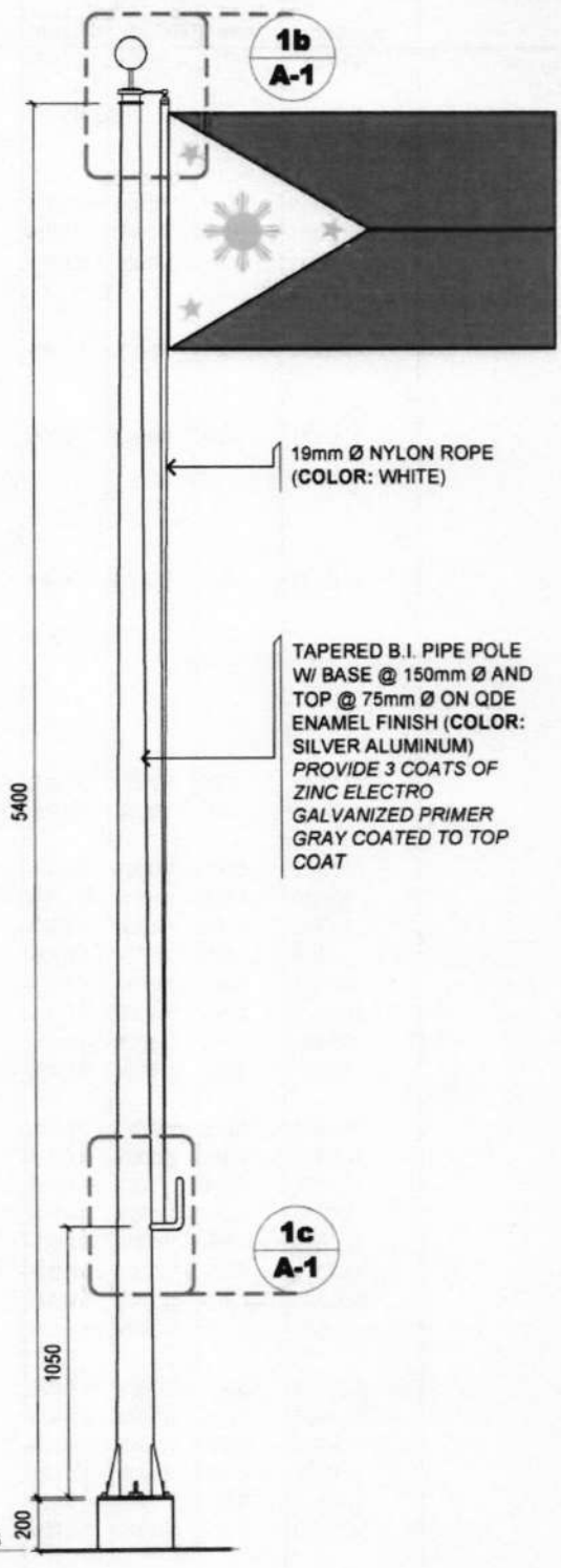
1a DETAILED ELEVATION SCALE 1:30 METERS
