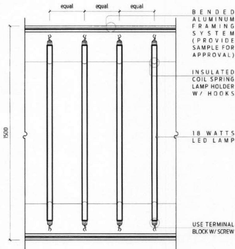
SECTION - A
