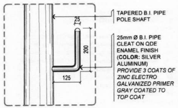
1c SPOT DETAIL - B SCALE 1:10 METERS
