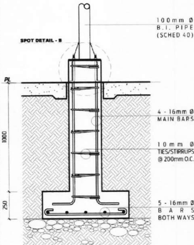
SECTION
