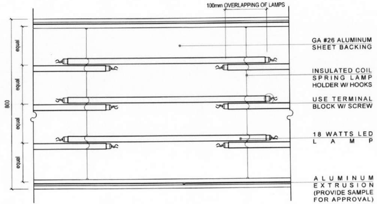
BLOW-UP SECTION-1 SCALE: 1:10 M
